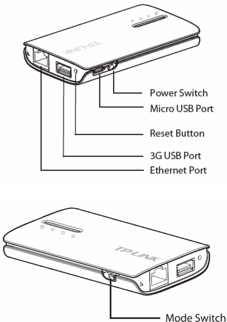
Figure 1-2 Rear Panel sketch
